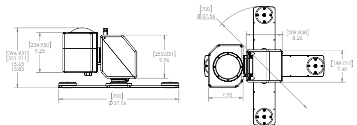
UW-HOU-A9 Dimensions
