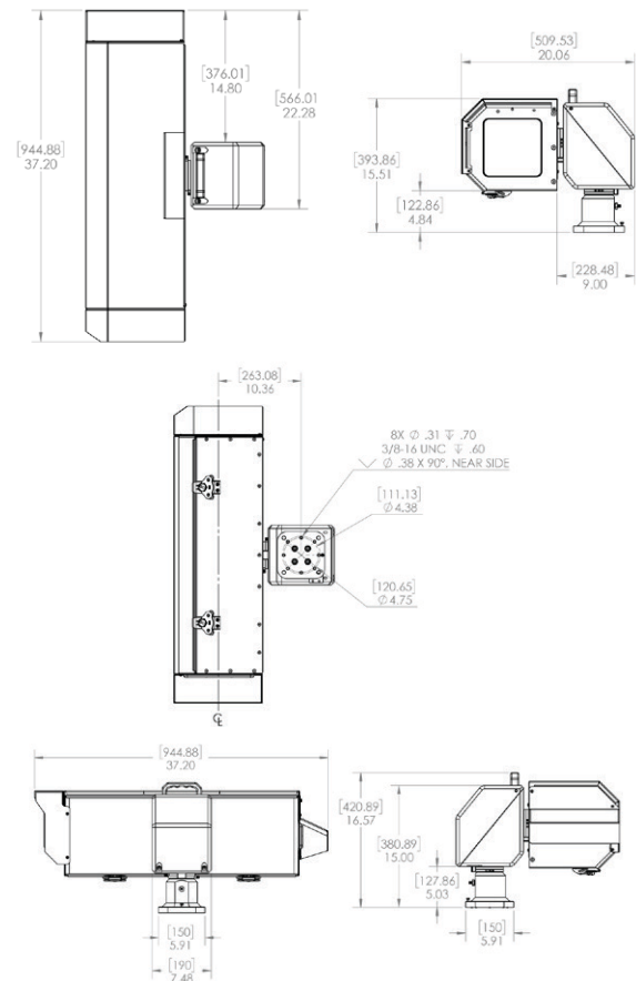
UW-HOU-A9 Dimensions
